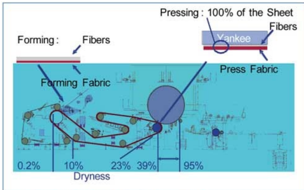
Picture 1: Example of Dry Crepe tissue technology with Crescent Former
